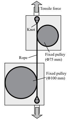
Fig. 4. Measurement of breaking strength after endurance test.
