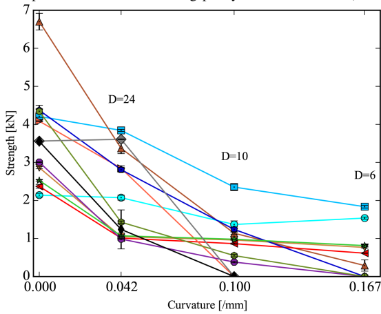
Fig. 11. Relation between test pulley diameter and tensile strength. (Tension: 31.3N, number of repetitions: 70 \times 10^3 )
